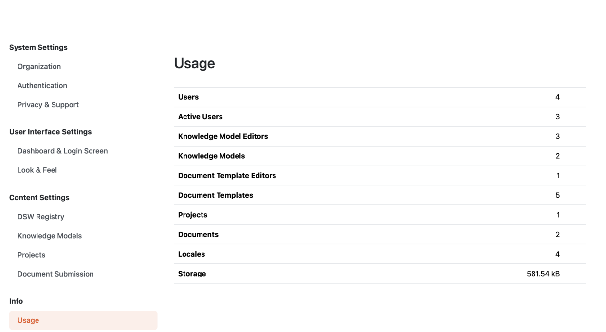
Fig. 68: Usage statistics.
