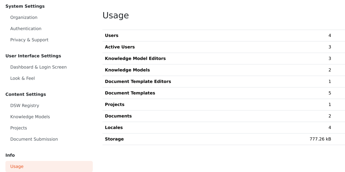
Fig. 68: Usage statistics.
